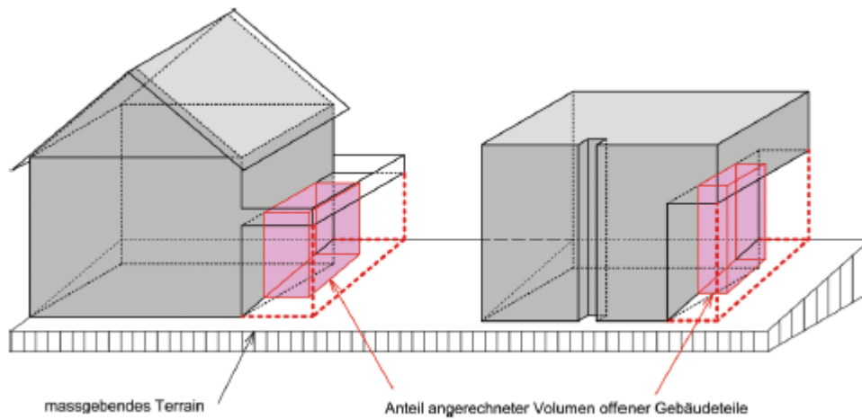
Fig. 8.3 Baumassenziffer
