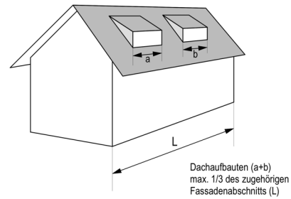
Giebellukarne
