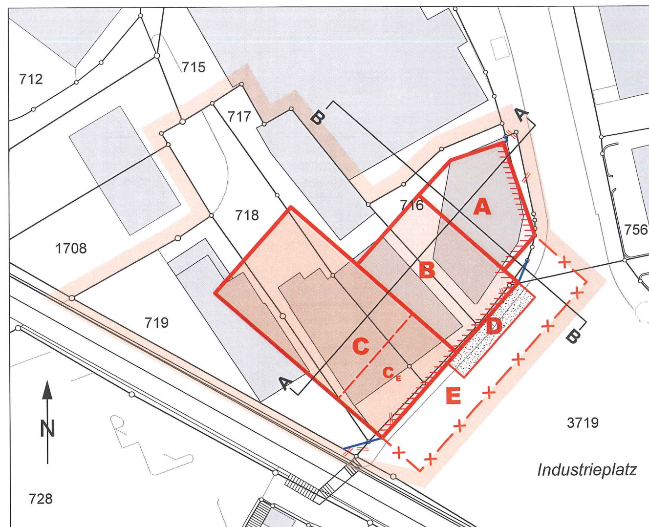
Situation 1:500
